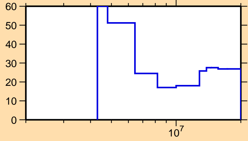
\Delta\sigma/\sigma vs. E for ^{32}\text{P}(n,n\text{cont.})
