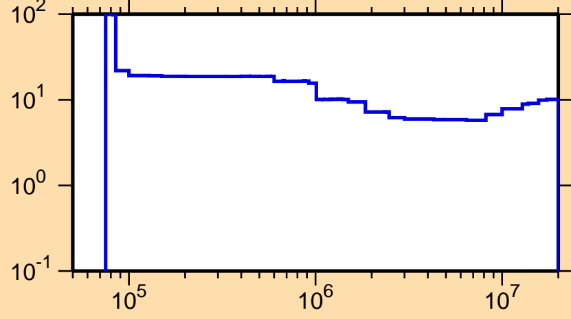
\Delta\sigma/\sigma vs. E for ^{32}\text{P}(n,\text{nonel.})
