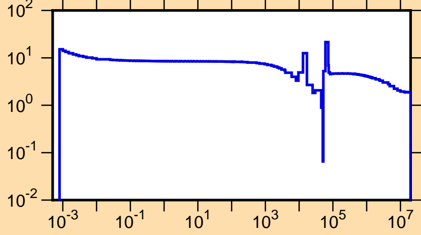
\sigma vs. E for ^{32}\text{P}(n,\text{tot.})
