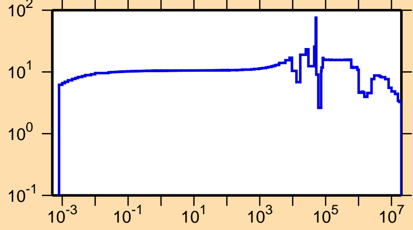
\Delta\sigma/\sigma vs. E for ^{32}\text{P}(n,\text{tot.})
