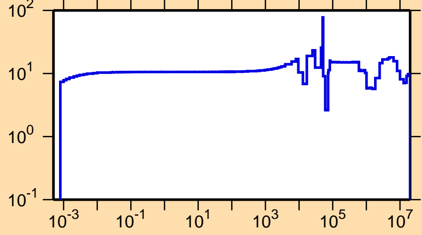
\Delta\sigma/\sigma vs. E for ^{32}\text{P}(n,\text{el.})
