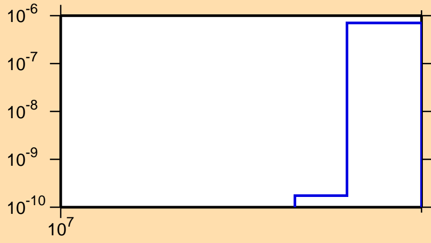
\sigma vs. E for ^{32}\text{P}(n,\text{He}3)
