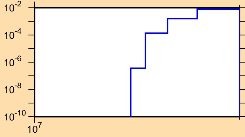
\sigma vs. E for ^{32}\text{P}(n,nd)
