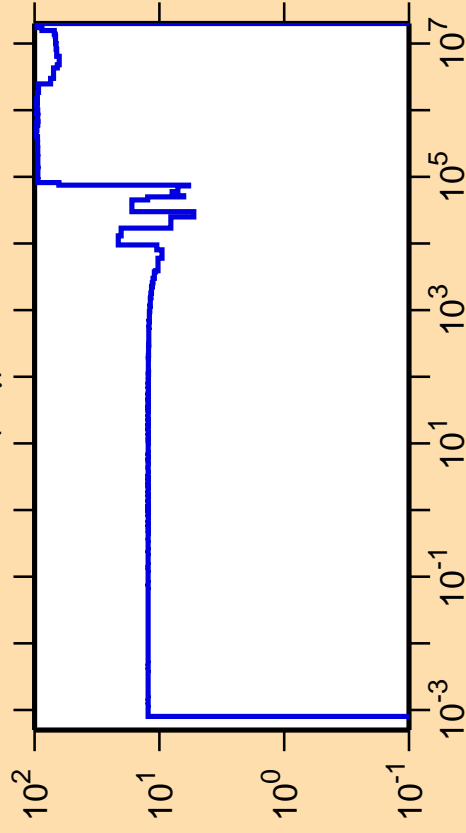
\Delta\sigma/\sigma vs. E for ^{32}\text{P}(n,\gamma)
