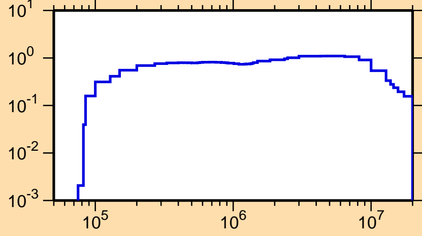
\sigma vs. E for ^{32}\text{P}(n,\text{inel.})
