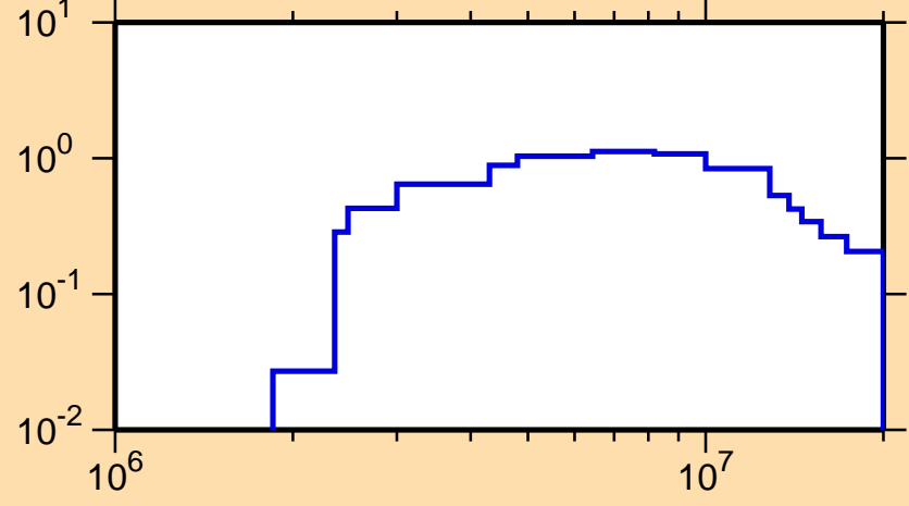
\sigma vs. E for ^{38}\text{Ar}(n,\text{inel.})
