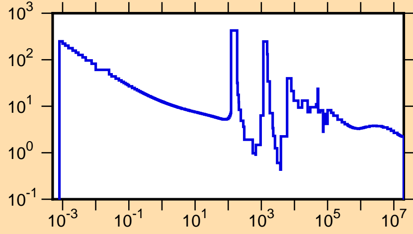
\sigma vs. E for ^{50}\text{V}(n,\text{tot.})
