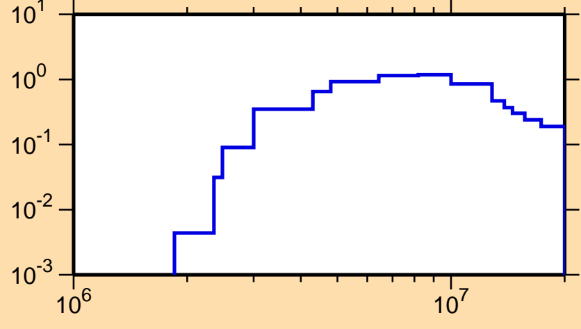
\sigma vs. E for ^{50}\text{V}(n,n\text{cont.})
