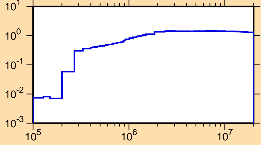
\sigma vs. E for ^{50}\text{V}(n,\text{nonel.})
