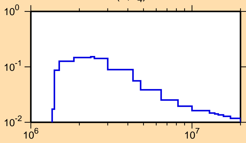
\sigma vs. E for ^{51}\text{Cr}(n,n_4)
