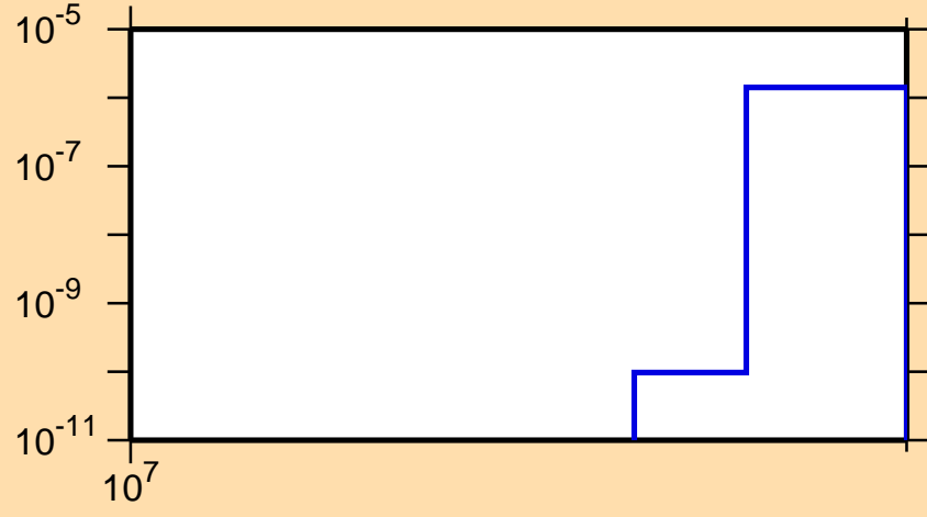
\sigma vs. E for ^{51}\text{Cr}(n,\text{pd})
