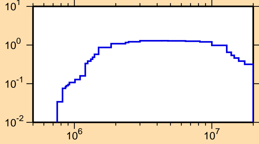
\sigma vs. E for ^{51}\text{Cr}(n,\text{inel.})
