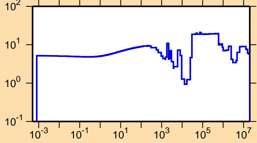
\Delta\sigma/\sigma vs. E for ^{52}\text{Mn}(n,\text{tot.})
