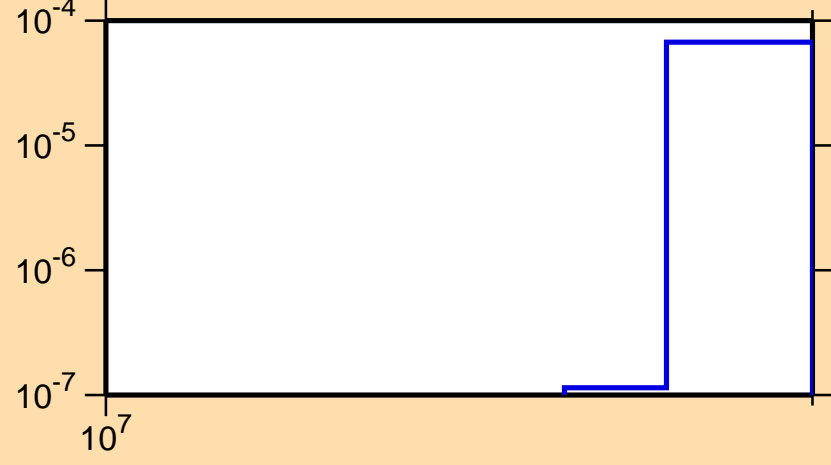
\sigma vs. E for ^{52}\text{Mn}(n,pd)
