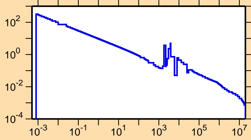
\sigma vs. E for ^{52}\text{Mn}(n,\gamma)
