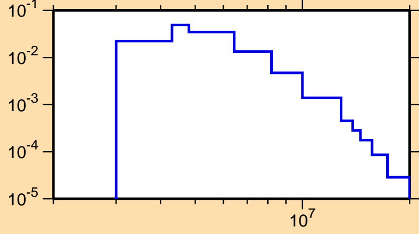
\sigma vs. E for ^{50}\text{Cr}(n,n_g)
