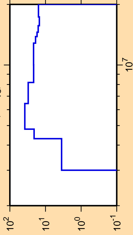
\Delta\sigma/\sigma vs. E for ^{50}\text{Cr}(n,n_{18})
