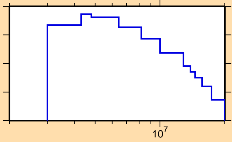
\sigma vs. E for ^{50}\text{Cr}(n,n_7)
