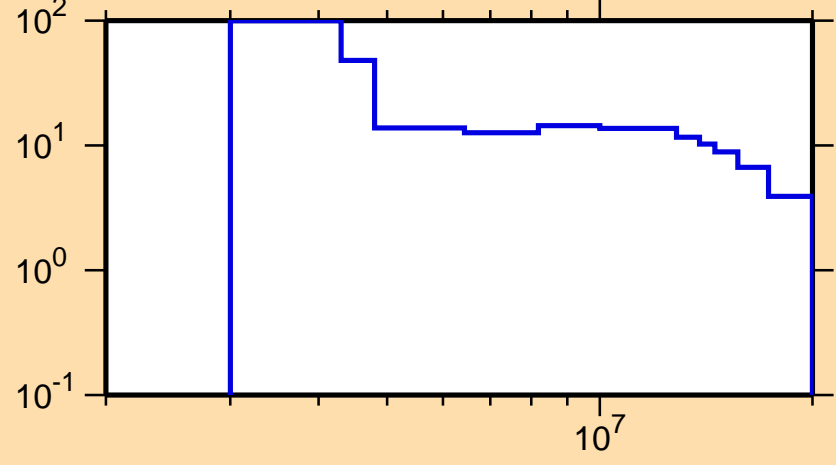
\Delta\sigma/\sigma vs. E for ^{50}\text{Cr}(\text{mt } 5)
