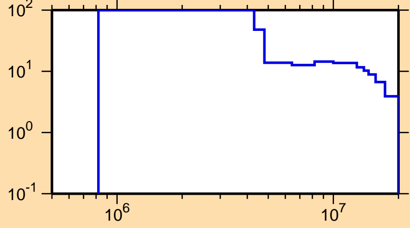
\Delta\sigma/\sigma vs. E for ^{50}\text{Cr}(mt\ 5)
