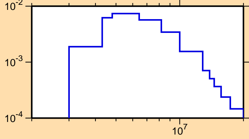
\sigma vs. E for ^{50}\text{Cr}(n,n_5)
