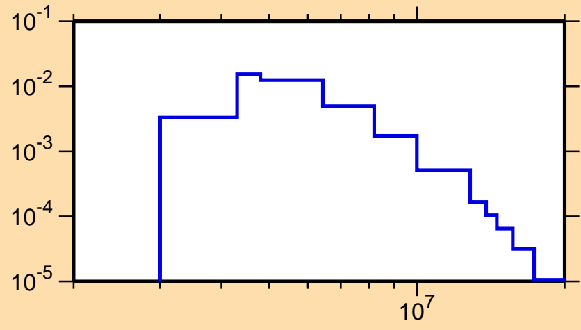
\sigma vs. E for ^{50}\text{Cr}(n,n_{18})
