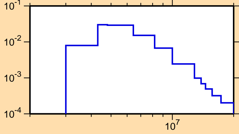
\sigma vs. E for ^{50}\text{Cr}(n,n_9)
