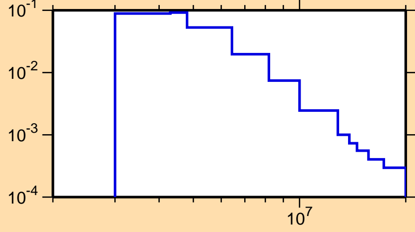
\sigma vs. E for ^{50}\text{Cr}(n,n_4)
