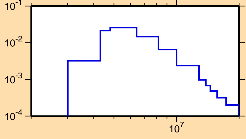
\sigma vs. E for ^{50}\text{Cr}(n,n_{15})
