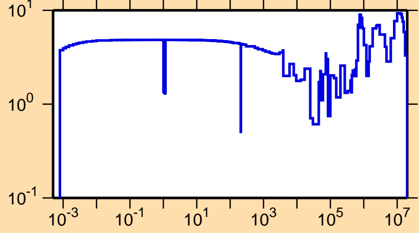
\Delta\sigma/\sigma vs. E for ^{50}\text{Cr}(n,\text{el.})
