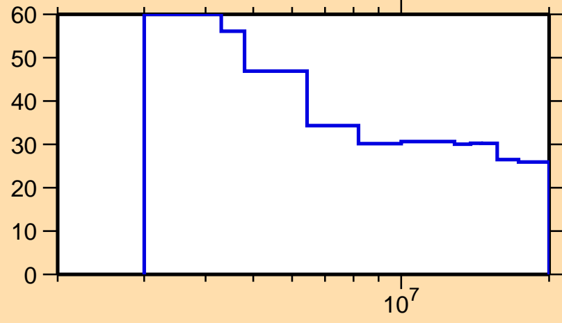
\Delta\sigma/\sigma vs. E for ^{57}\text{Ni}(n,ncont.)
