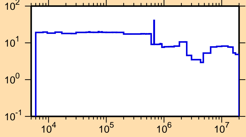
\Delta\sigma/\sigma vs. E for ^{57}\text{Ni}(n,\text{tot.})
