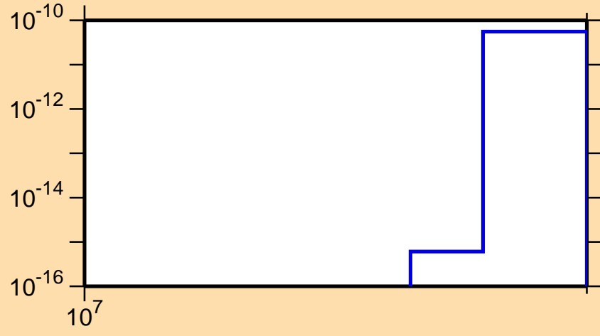
\sigma vs. E for ^{67}\text{Zn}(n,pd)
