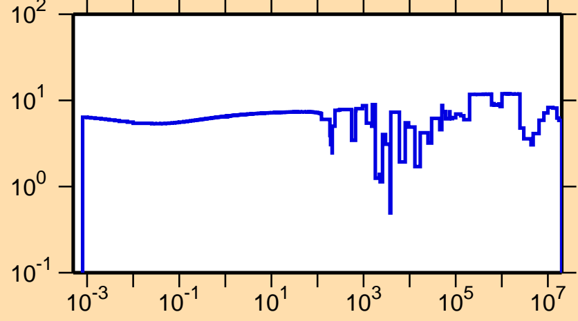
\Delta\sigma/\sigma vs. E for ^{67}\text{Zn}(n,\text{tot.})
