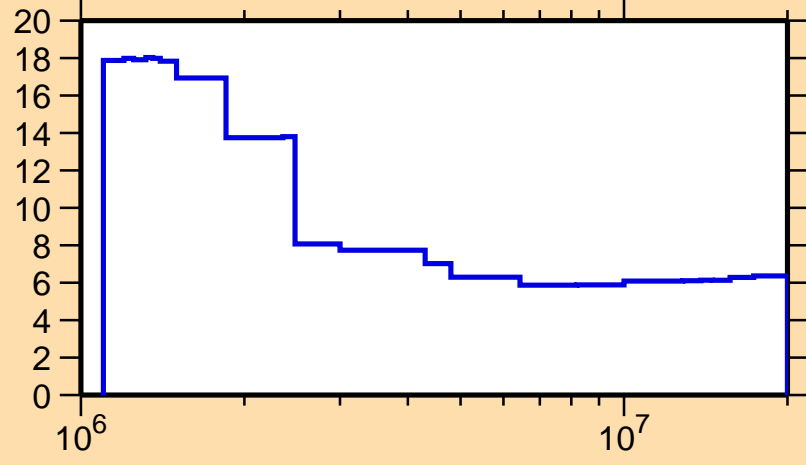
\Delta\sigma/\sigma vs. E for ^{73}\text{Ge}(n,n\text{onel.})
