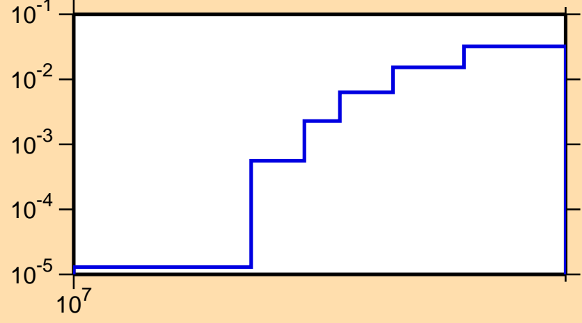
\sigma vs. E for ^{73}\text{Ge}(n,np)
