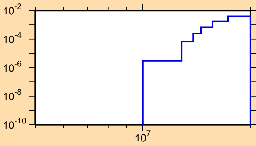
\sigma vs. E for ^{73}\text{Ge}(n,t)
