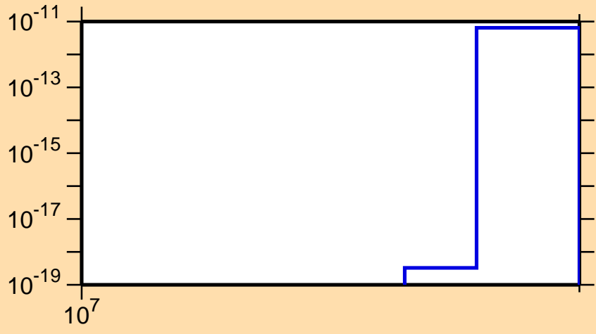
\sigma vs. E for ^{71}\text{As} (mt 34)
