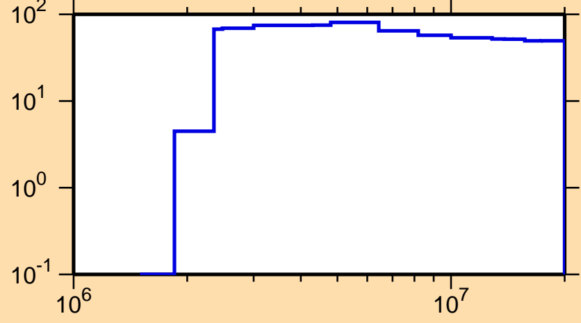
\Delta\sigma/\sigma vs. E for ^{79}\text{Se}(n,p)
