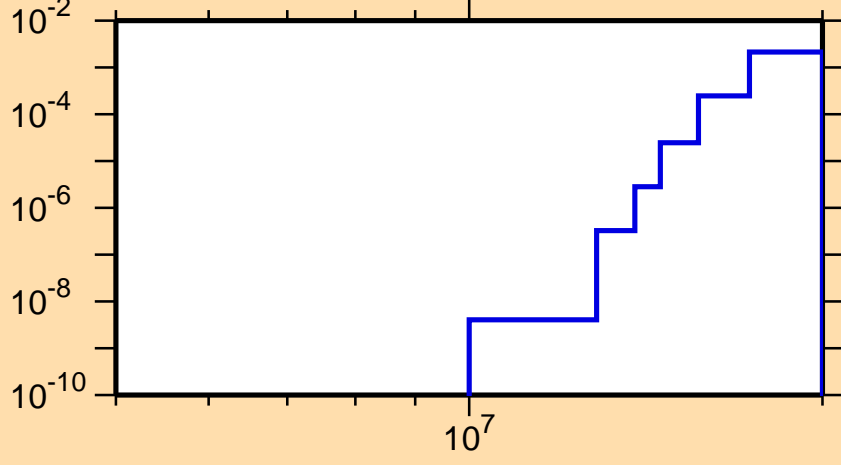
\sigma vs. E for ^{88}\text{Rb}(n,\alpha)
