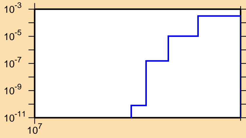
\sigma vs. E for ^{88}\text{Rb}(n,nd)
