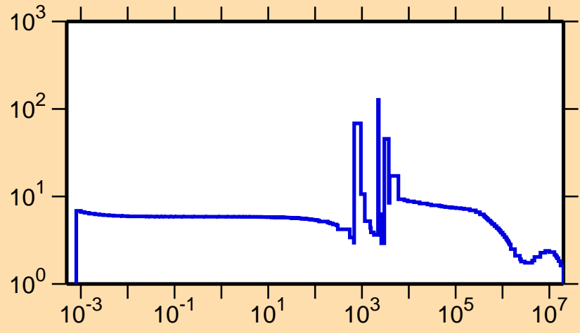
\sigma vs. E for ^{88}\text{Rb}(n,\text{el.})
