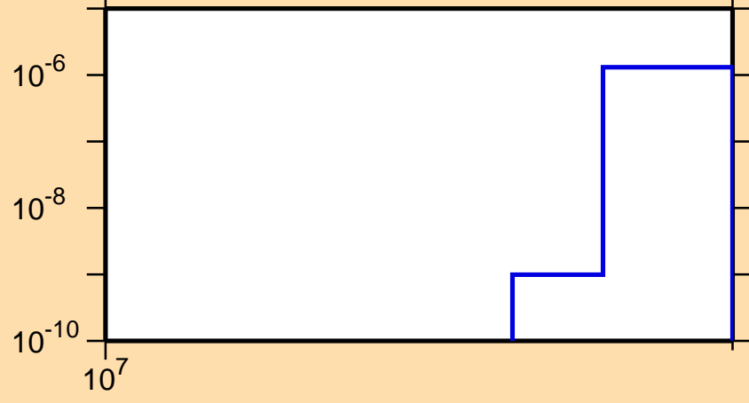
\sigma vs. E for ^{84}\text{Sr}(n,\text{pd})
