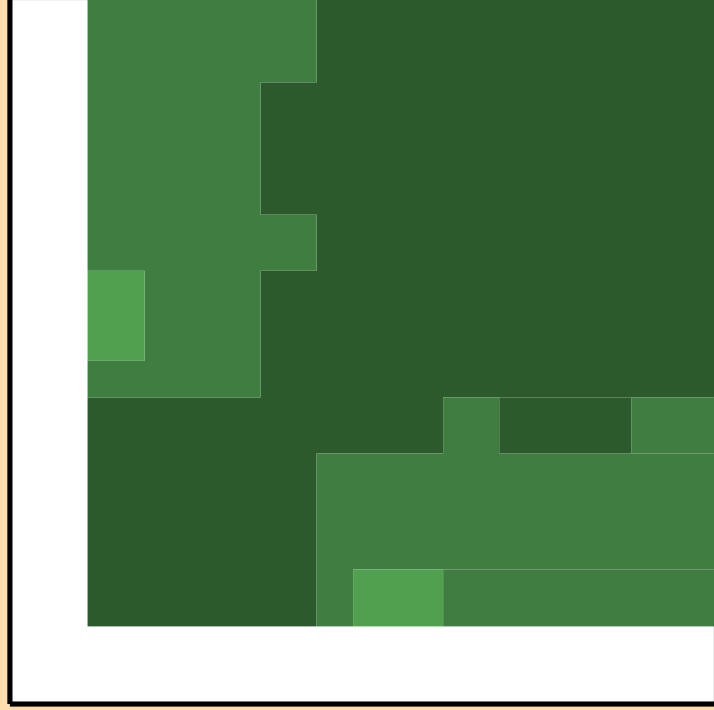
\sigma vs. E for ^{84}\text{Sr}(n,n_1)
