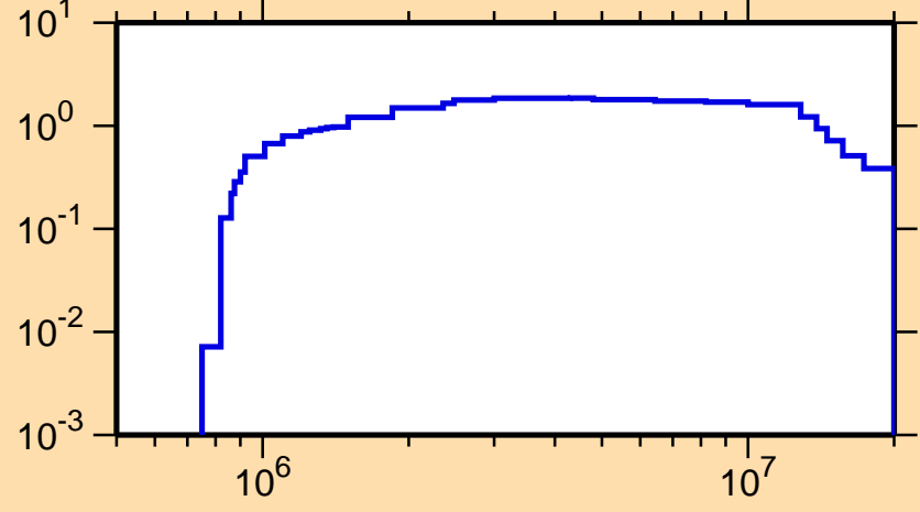
\sigma vs. E for ^{84}\text{Sr}(n,\text{inel.})
