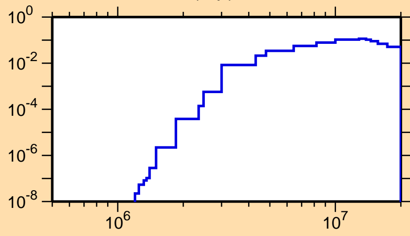
\sigma vs. E for ^{84}\text{Sr}(n,p)
