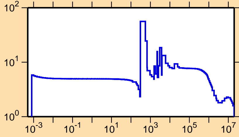
\sigma vs. E for ^{84}\text{Sr}(n,\text{el.})
