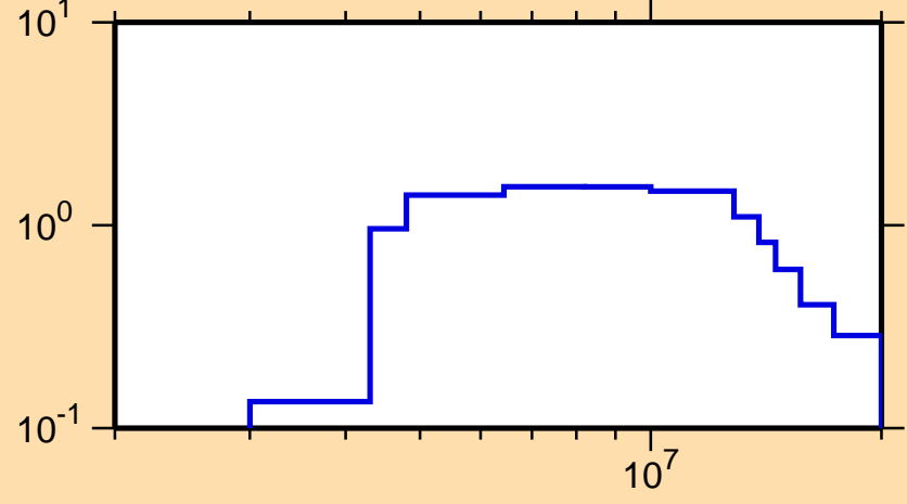
\sigma vs. E for ^{84}\text{Sr}(n,n\text{cont.})
