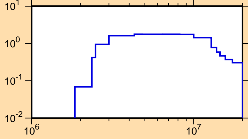
\sigma vs. E for ^{85}\text{Rb}(n,n\text{cont.})
