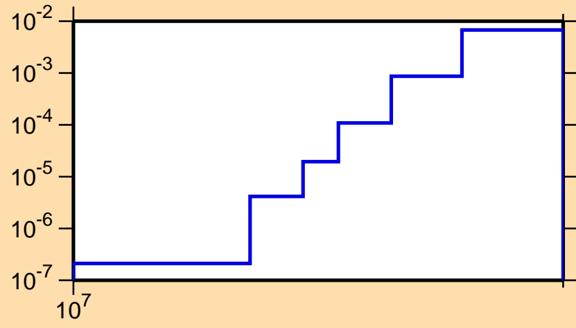
\sigma vs. E for ^{90}\text{Zr}(n,\alpha)
