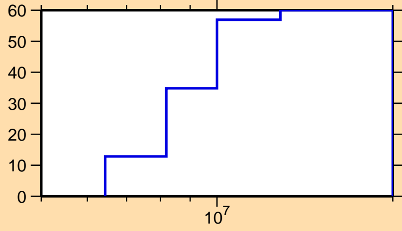
\Delta\sigma/\sigma vs. E for ^{90}\text{Sr}(n,ncont.)
