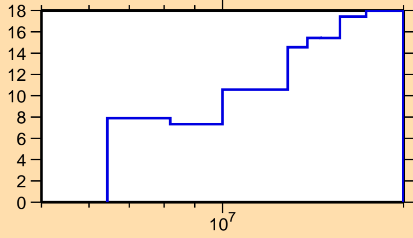
\Delta\sigma/\sigma vs. E for ^{90}\text{Sr}(n,el.)
