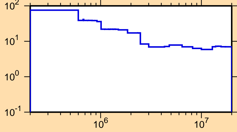
\Delta\sigma/\sigma vs. E for ^{90}\text{Sr}(n,\text{nonel.})
