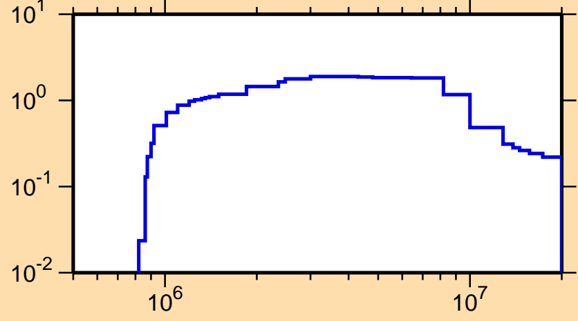
\sigma vs. E for ^{90}\text{Sr}(n,\text{inel.})
