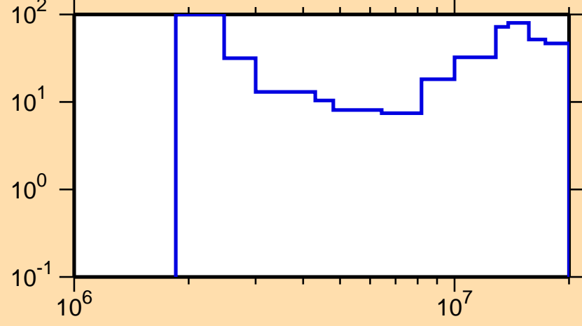
\Delta\sigma/\sigma vs. E for ^{87}\text{Y}(n,ncont.)
