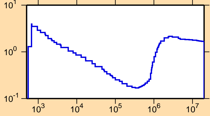
\sigma vs. E for ^{87}\text{Y}(n,\text{nonel.})
