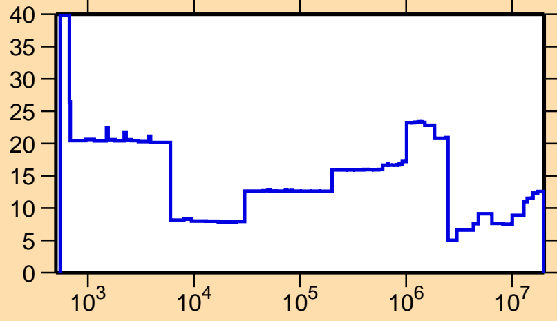
\Delta\sigma/\sigma vs. E for ^{87}\text{Y}(n,el.)
