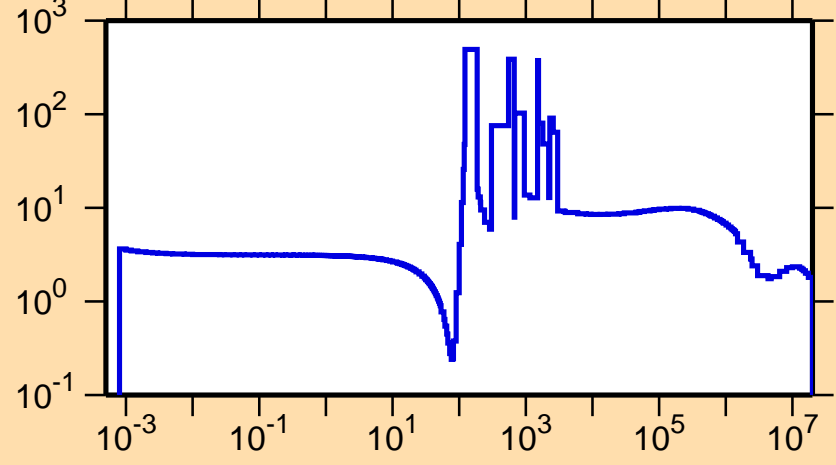
\sigma vs. E for ^{93}\text{Mo}(n,\text{el.})
