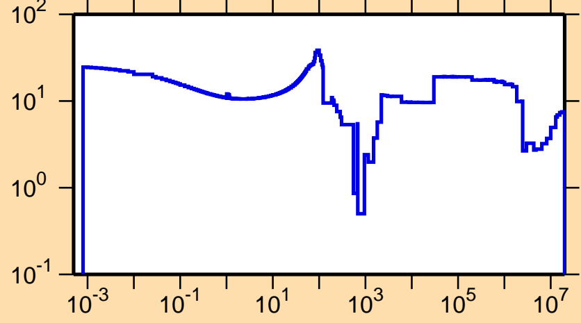
\Delta\sigma/\sigma vs. E for ^{93}\text{Mo}(n,\text{tot.})
