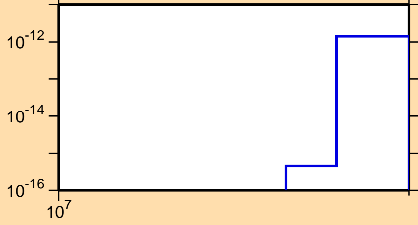
\sigma vs. E for ^{93}\text{Mo}(\text{mt117})
