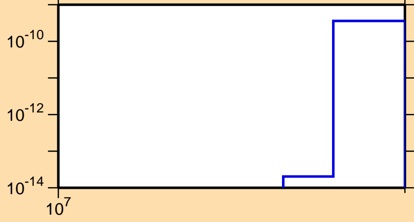
\sigma vs. E for ^{100}\text{Ru}(n,\text{pd})
