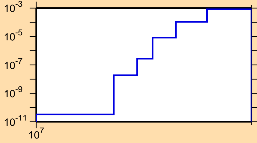
\sigma vs. E for ^{100}\text{Ru}(n,t)
