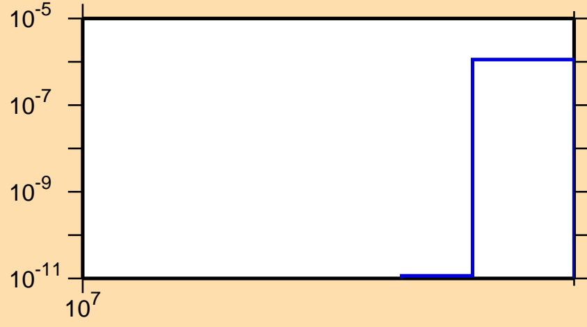
\sigma vs. E for ^{100}\text{Ru}(n,\text{nd})
