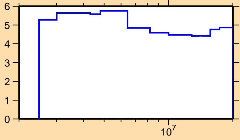
\Delta\sigma/\sigma vs. E for ^{100}\text{Ru}(n,n\text{onel.})
