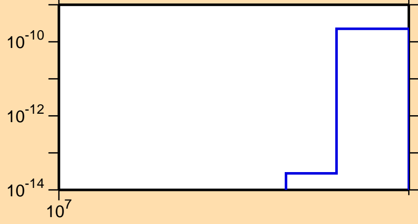
\sigma vs. E for ^{101}\text{Rh}(n,\text{pd})
