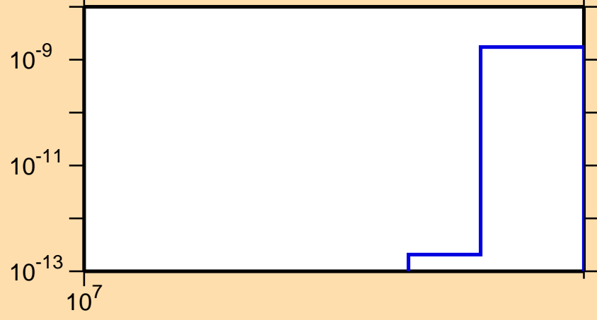
\sigma vs. E for ^{106}\text{Ru}(n,\text{nd})
