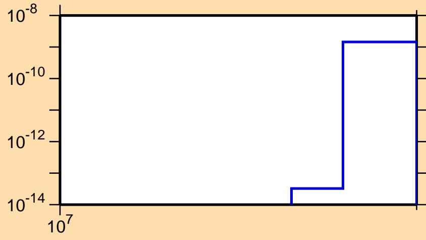
\sigma vs. E for ^{106}\text{Ru}(n,2n\alpha)
