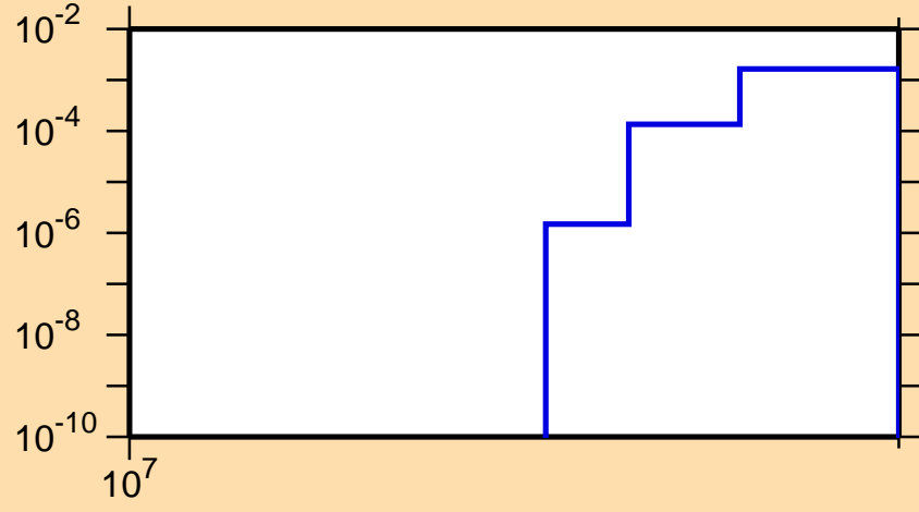
\sigma vs. E for ^{108}\text{Ag}(n,2np)
