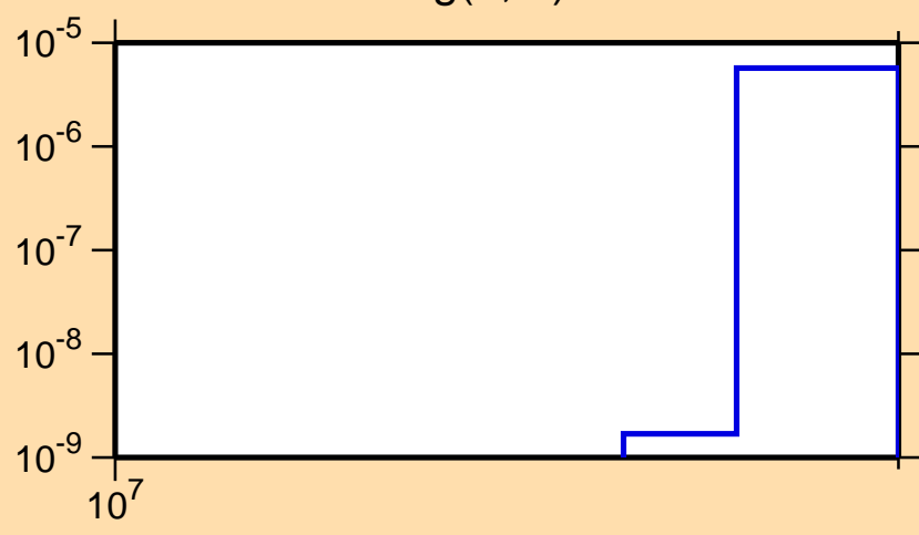
\sigma vs. E for ^{108}\text{Ag}(n,nt)
