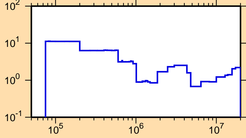
\Delta\sigma/\sigma vs. E for ^{108}\text{Ag}(n,\text{tot.})
