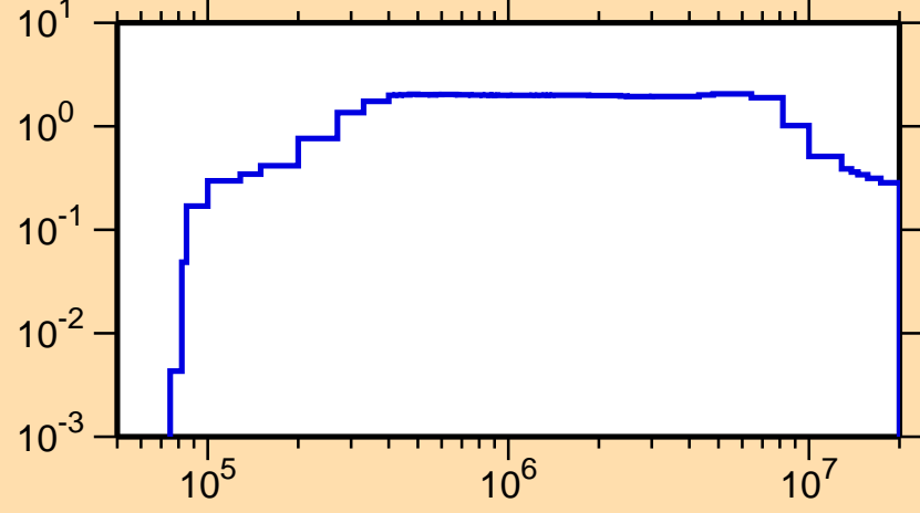
\sigma vs. E for ^{108}\text{Ag}(n,\text{inel.})
