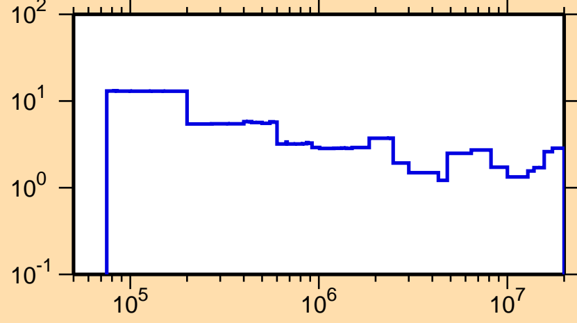
\Delta\sigma/\sigma vs. E for ^{108}\text{Ag}(n,\text{el.})
