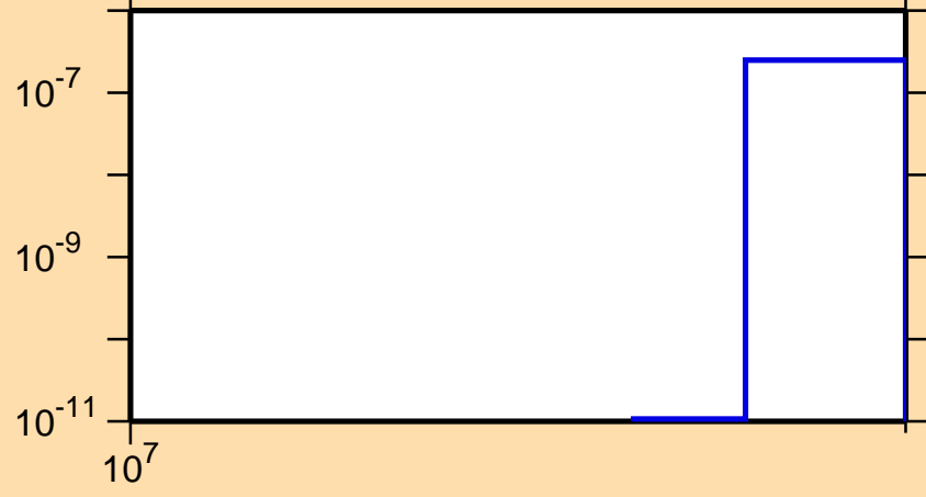
\sigma vs. E for ^{131}\text{Te}(n,2np)
