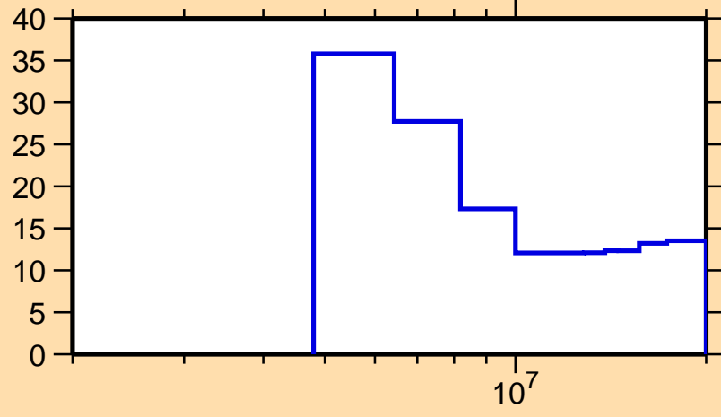
\Delta\sigma/\sigma vs. E for ^{132}\text{Te}(n,el.)
