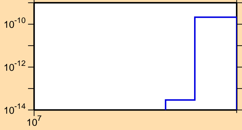
\sigma vs. E for ^{132}\text{Te}(n,2n\alpha)
