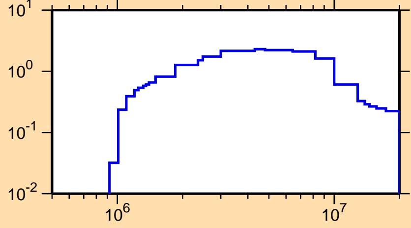
\sigma vs. E for ^{132}\text{Te}(n,\text{inel.})
