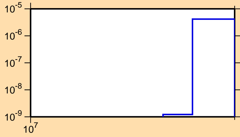
\sigma vs. E for ^{128}\text{I}(n,nt)
