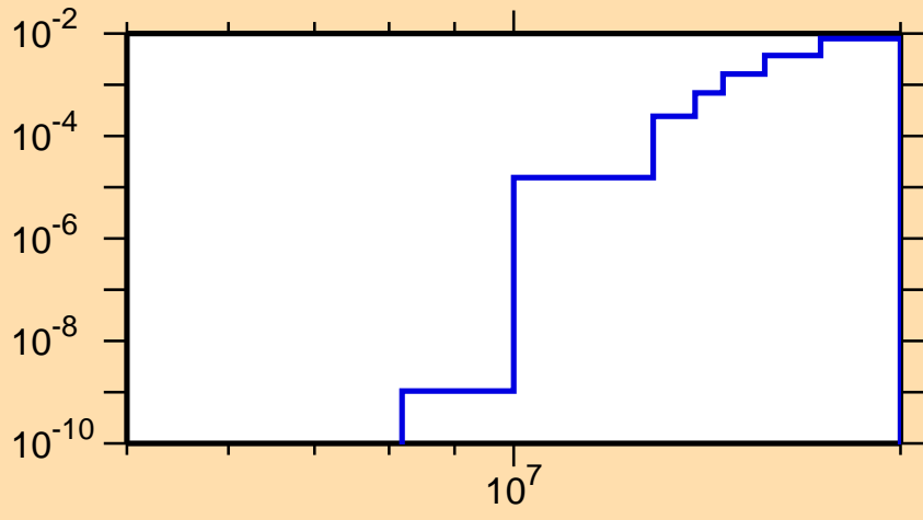
\sigma vs. E for ^{124}\text{Te}(n,d)
