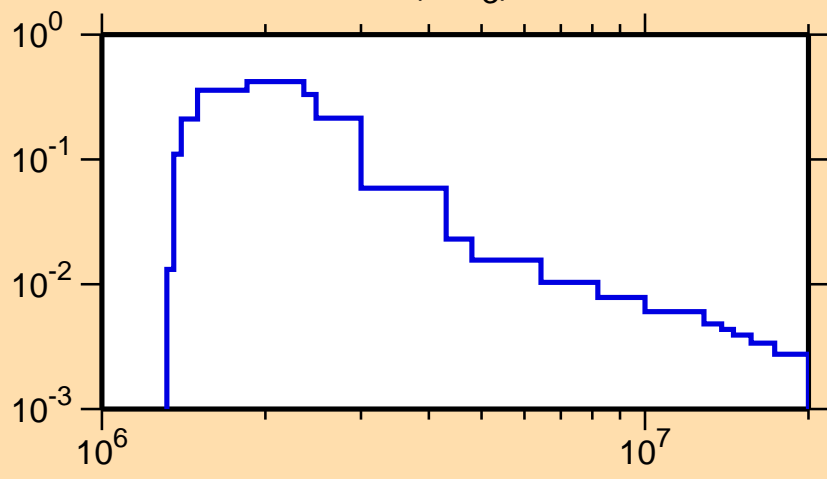
\sigma vs. E for ^{124}\text{Te}(n,n_3)
