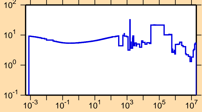
\Delta\sigma/\sigma vs. E for ^{124}\text{Te}(n,\text{tot.})
