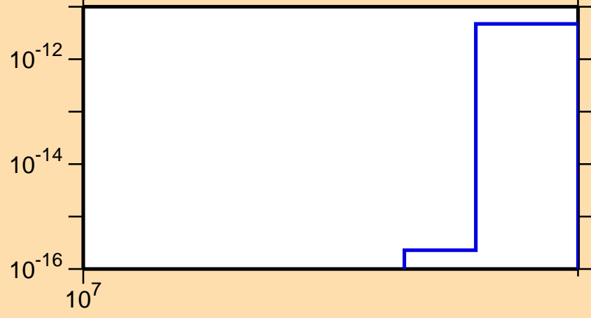
\sigma vs. E for ^{124}\text{Te}(n,pd)
