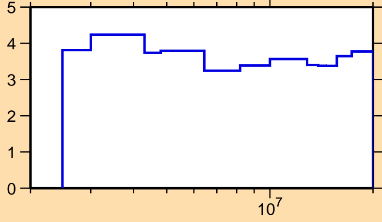
\Delta\sigma/\sigma vs. E for ^{124}\text{Te}(n,\text{nonel.})
