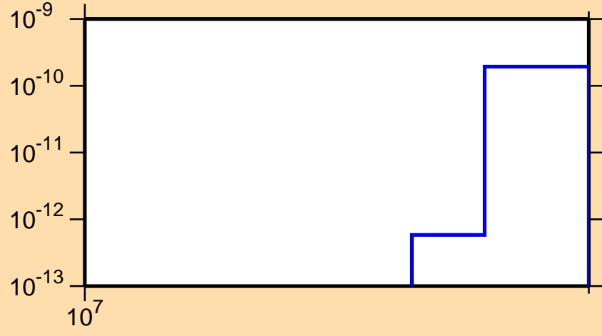
\sigma vs. E for ^{140}\text{Ba}(\text{mt117})
