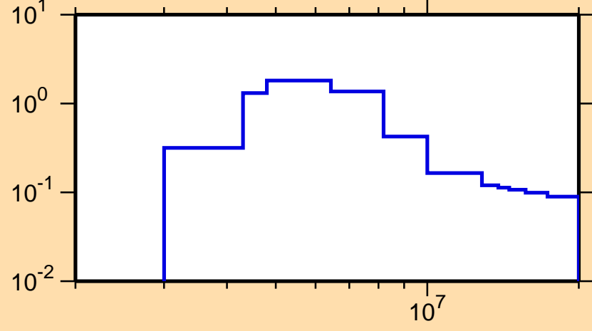
\sigma vs. E for ^{140}\text{Ba}(n,n\text{cont.})
