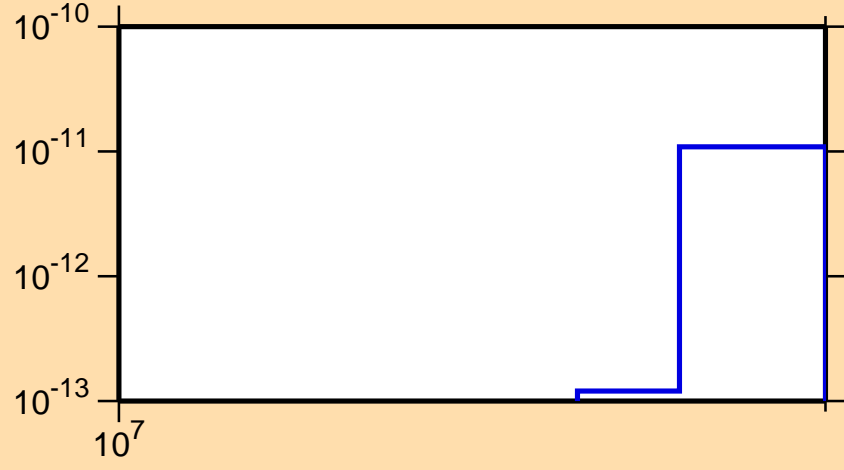
\sigma vs. E for ^{140}\text{Ba}(n,p\alpha)
