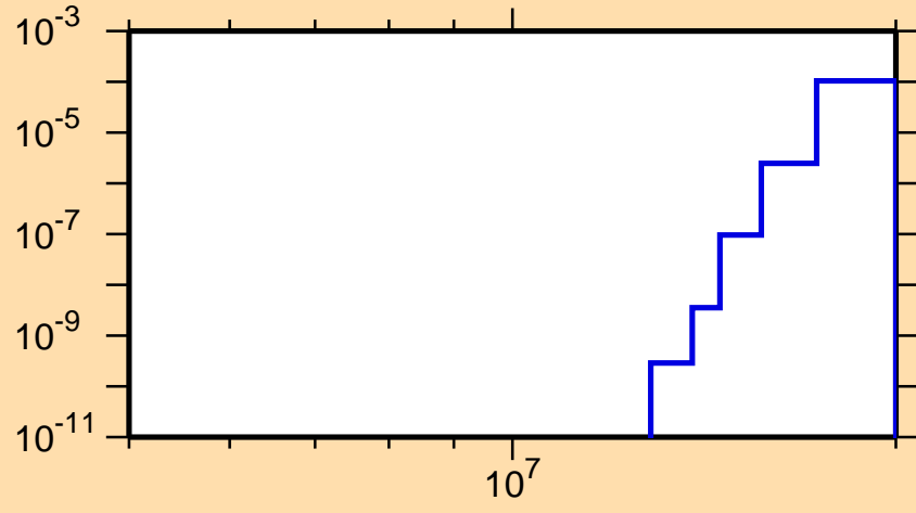
\sigma vs. E for ^{140}\text{Ba}(n,2n\alpha)
