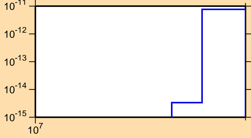
\sigma vs. E for ^{140}\text{Ba} (mt 45)
