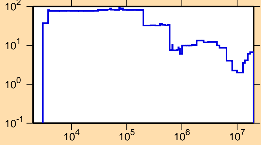
\Delta\sigma/\sigma vs. E for ^{142}\text{Pr}(n,\text{tot.})
