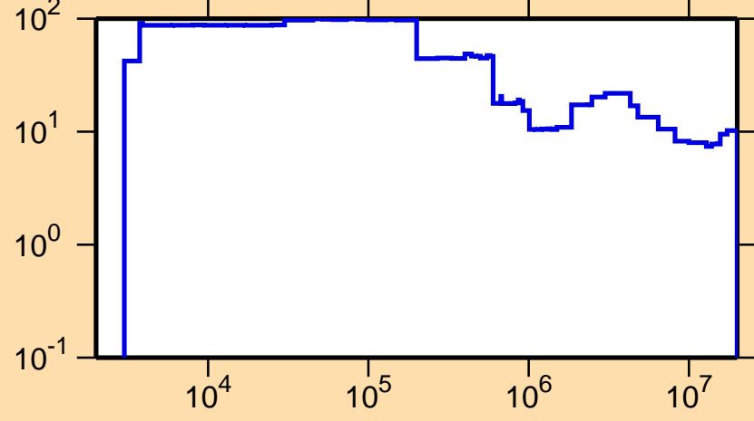
\Delta\sigma/\sigma vs. E for ^{142}\text{Pr}(n,\text{el.})
