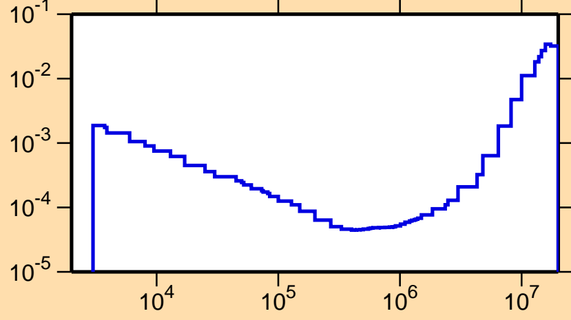
\sigma vs. E for ^{142}\text{Pr}(n,\alpha)
