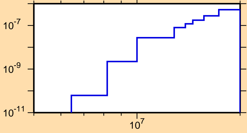
\sigma vs. E for ^{142}\text{Pr}(n,\rho\alpha)
