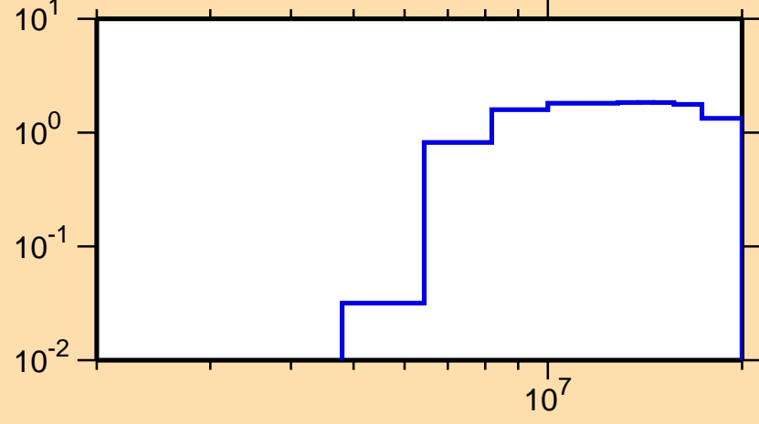
\sigma vs. E for ^{142}\text{Pr}(n,2n)
