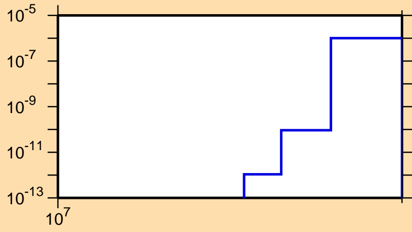
\sigma vs. E for ^{136}\text{Ce}(n,\text{nd})
