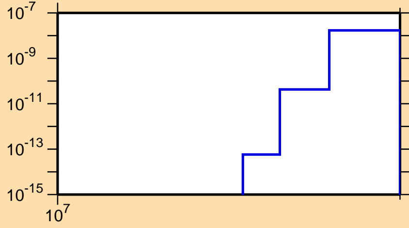
\sigma vs. E for ^{136}\text{Ce}(n,pd)
