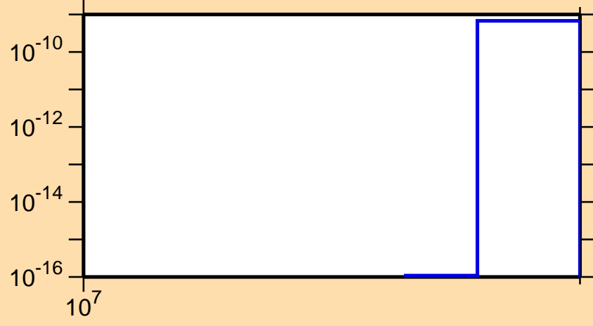
\sigma vs. E for ^{136}\text{Ce}(n,\text{nt})
