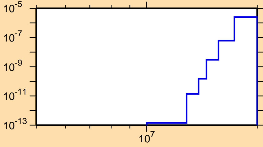
\sigma vs. E for ^{136}\text{Ce}(n,\text{He3})
