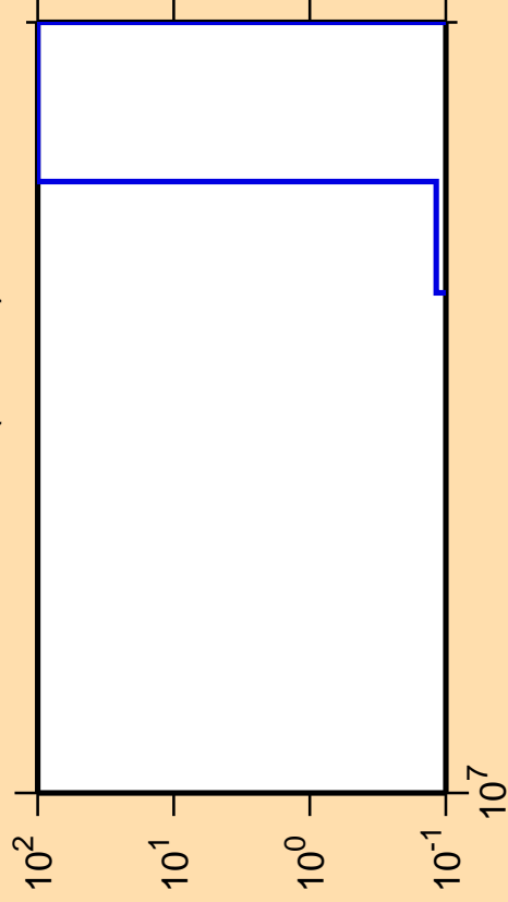
\Delta\sigma/\sigma vs. E for ^{136}\text{Ce} (mt 45)
