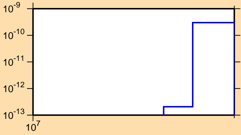
\sigma vs. E for ^{136}\text{Ce} (mt 45)
