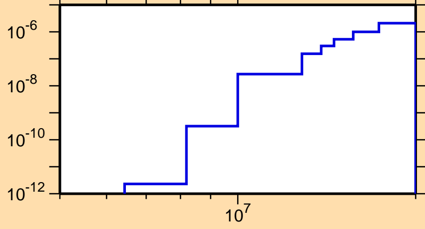
\sigma vs. E for ^{143}\text{Nd}(n,p\alpha)
