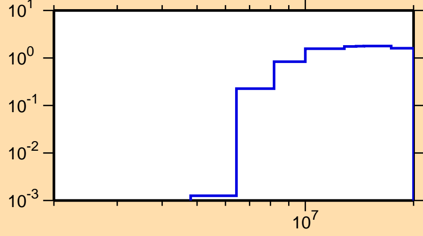
\sigma vs. E for ^{143}\text{Nd}(n,2n)
