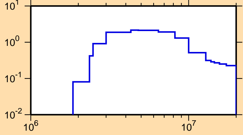
\sigma vs. E for ^{143}\text{Nd}(n,n\text{cont.})
