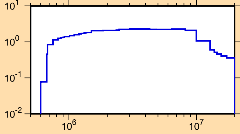
\sigma vs. E for ^{150}\text{Gd}(n,\text{inel.})
