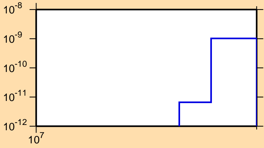
\sigma vs. E for ^{150}\text{Gd}(n,pd)
