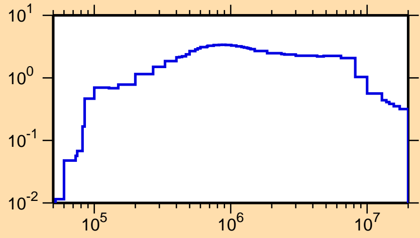
\sigma vs. E for ^{158}\text{Tb}(n,\text{inel.})
