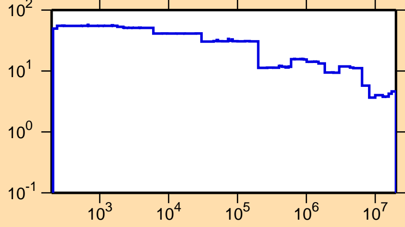
\Delta\sigma/\sigma vs. E for ^{158}\text{Tb}(n,\text{tot.})
