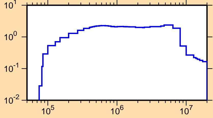
\sigma vs. E for ^{172}\text{Er}(n,\text{inel.})
