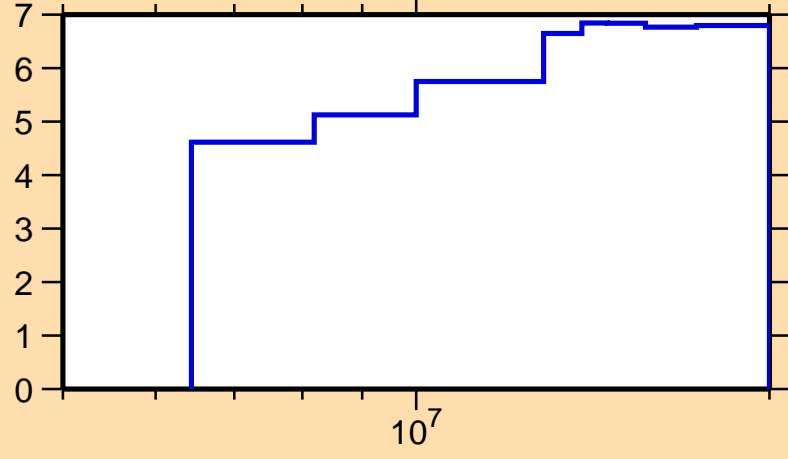
\Delta\sigma/\sigma vs. E for ^{172}\text{Er}(n,\text{nonel.})
