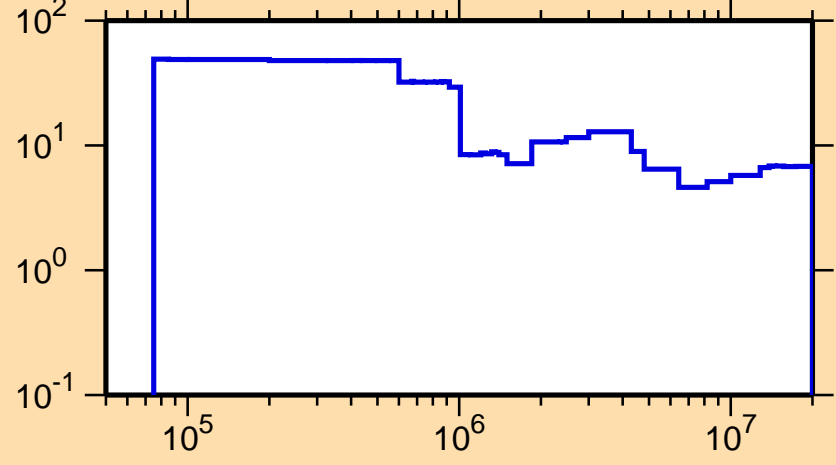
\Delta\sigma/\sigma vs. E for ^{172}\text{Er}(n,\text{nonel.})
