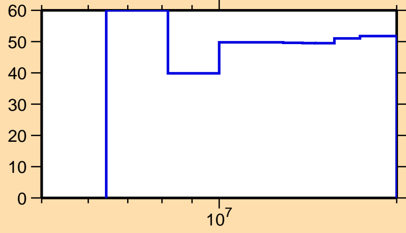
\Delta\sigma/\sigma vs. E for ^{172}\text{Er}(n,ncont.)
