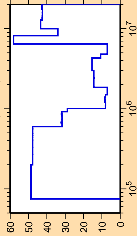
\Delta\sigma/\sigma vs. E for ^{172}\text{Er}(n,\text{inel.})
