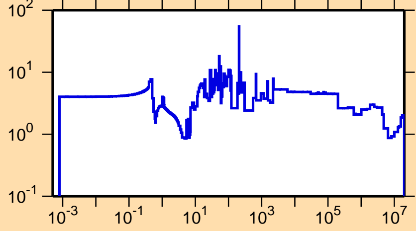
\Delta\sigma/\sigma vs. E for ^{167}\text{Er}(n,\text{tot.})
