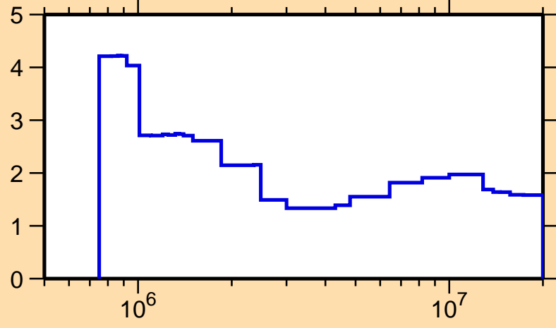
\Delta\sigma/\sigma vs. E for ^{167}\text{Er}(n,n\text{oncl.})
