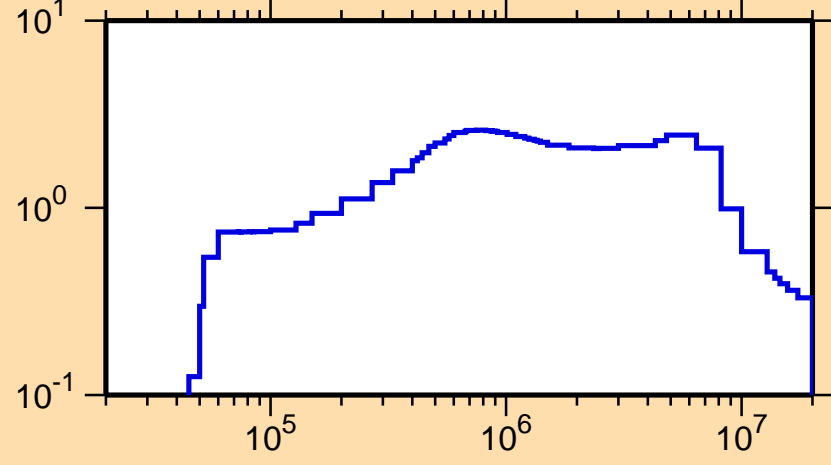
\sigma vs. E for ^{174}\text{Lu}(n,\text{inel.})
