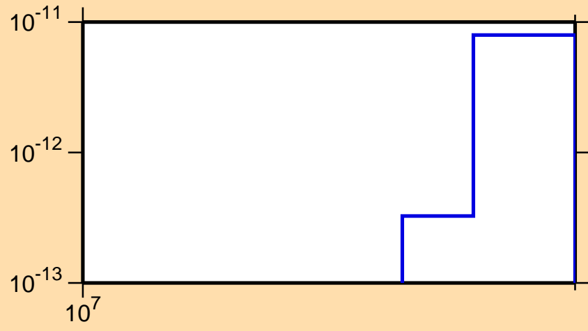
\sigma vs. E for ^{174}\text{Lu}(\text{mt117})
