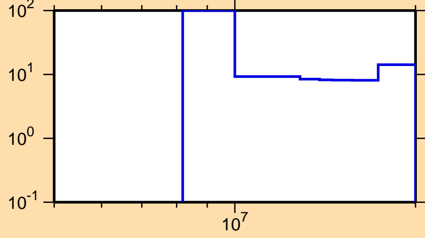
\Delta\sigma/\sigma vs. E for ^{176}\text{Hf}(n,2n)
