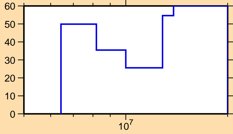
\Delta\sigma/\sigma vs. E for ^{176}\text{Hf}(n,\gamma)
