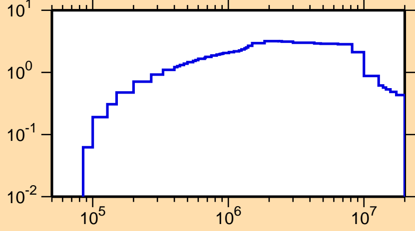
\sigma vs. E for ^{176}\text{Hf}(n,\text{inel.})
