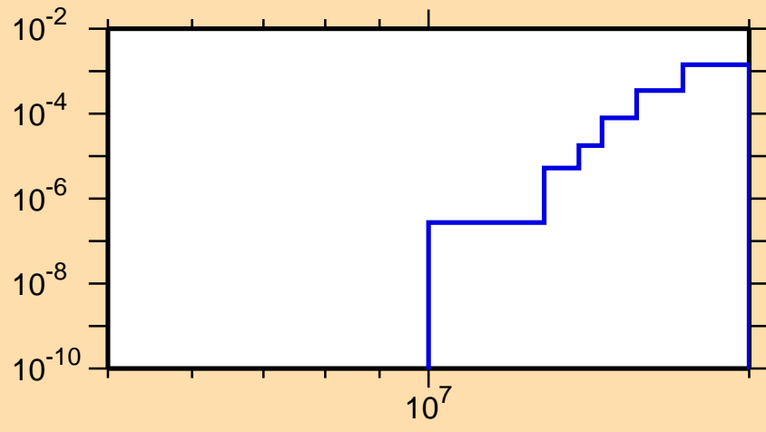
\sigma vs. E for ^{182}\text{W}(n,t)
