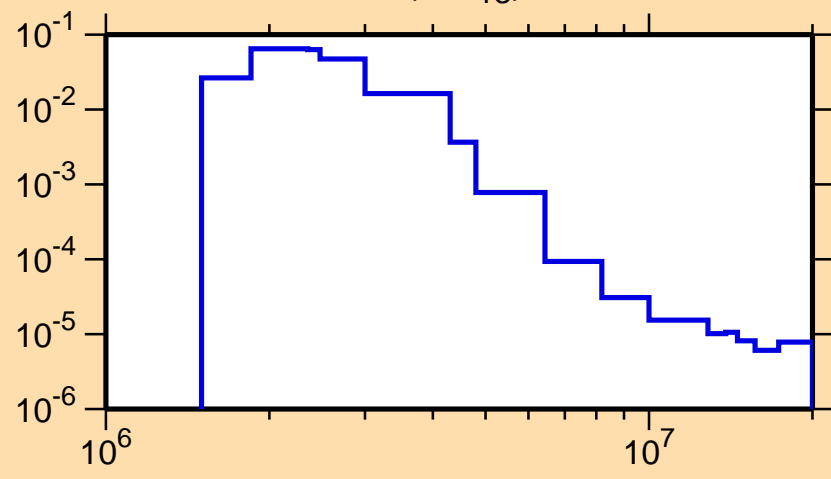
\sigma vs. E for ^{182}\text{W}(n,n_{13})
