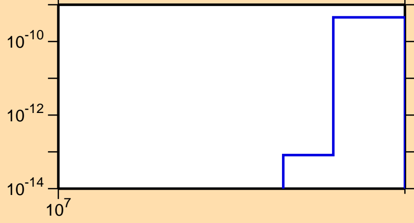
\sigma vs. E for ^{188}\text{Re}(n,3n\alpha)
