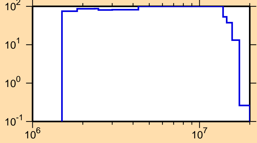
\Delta\sigma/\sigma vs. E for ^{188}\text{Re}(n,n_1)
