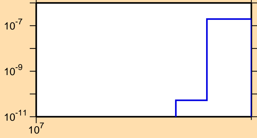
\sigma vs. E for ^{188}\text{W}(n,\text{nd})
