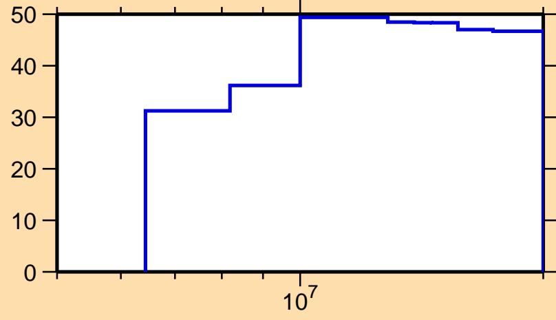
\Delta\sigma/\sigma vs. E for ^{188}\text{W}(n,ncont.)
