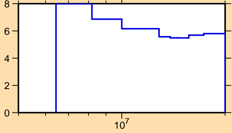
\Delta\sigma/\sigma vs. E for ^{188}\text{W}(n,\text{nonel.})
