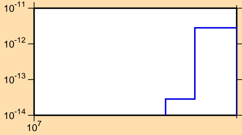
\sigma vs. E for ^{169}\text{Tm} (mt 45)
