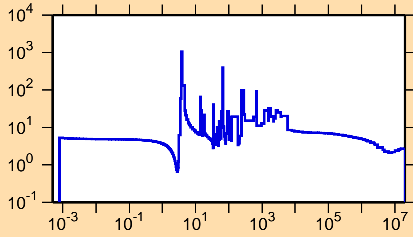
\sigma vs. E for ^{169}\text{Tm}(n,\text{el.})
