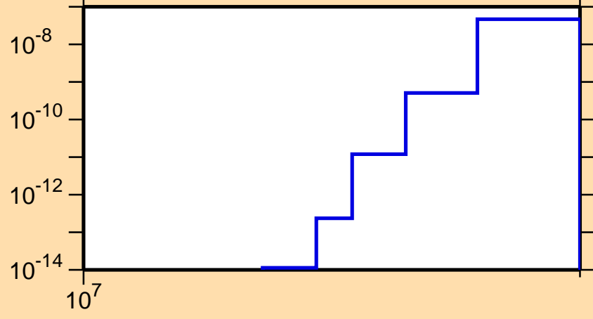
\sigma vs. E for ^{169}\text{Tm}(n,\text{He}3)
