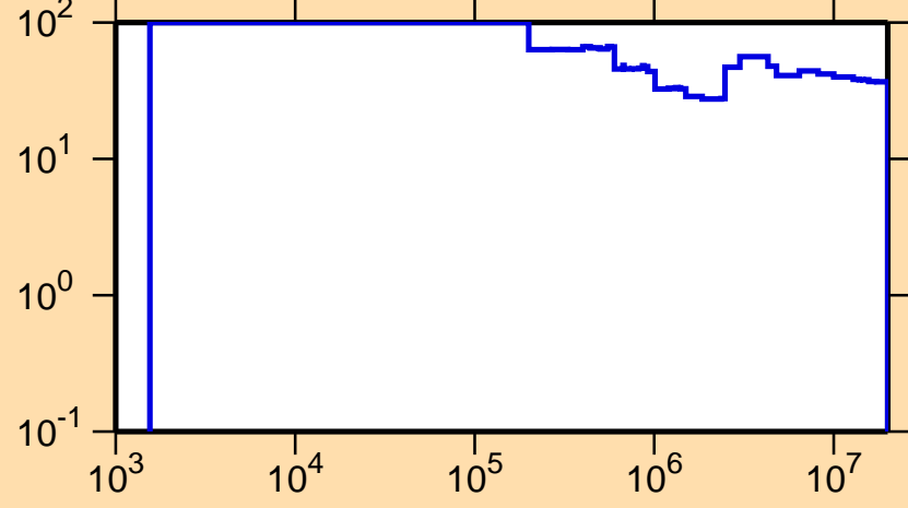
\Delta\sigma/\sigma vs. E for ^{201}\text{Hg}(n,n_1)
