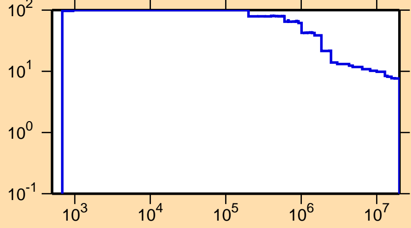
\Delta\sigma/\sigma vs. E for ^{201}\text{Hg}(n,\text{nonel.})
