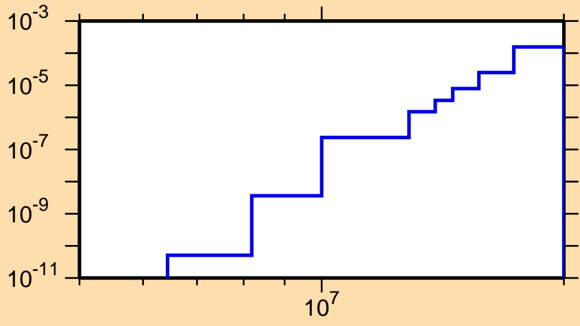
\sigma vs. E for ^{201}\text{Hg}(n,\alpha)
