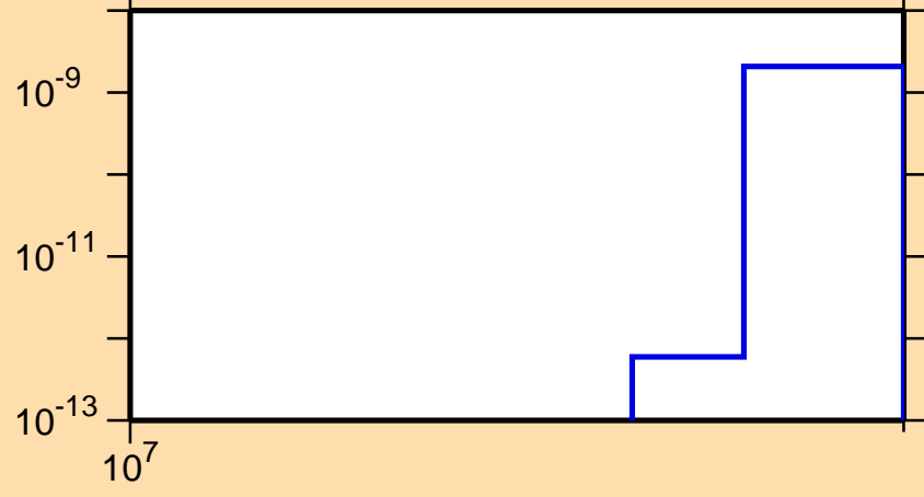
\sigma vs. E for ^{188}\text{Os}(n,3n\alpha)
