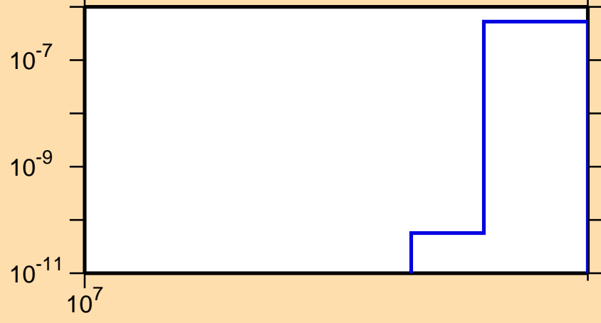
\sigma vs. E for ^{188}\text{Os}(n,2np)
