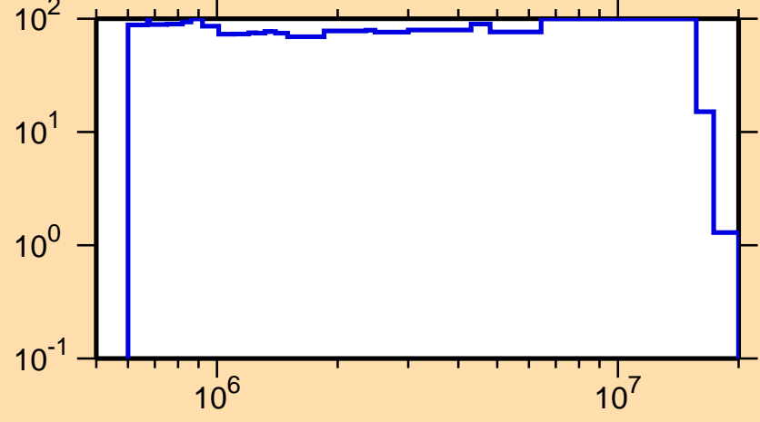
\Delta\sigma/\sigma vs. E for ^{191}\text{Os}(n,n_1)
