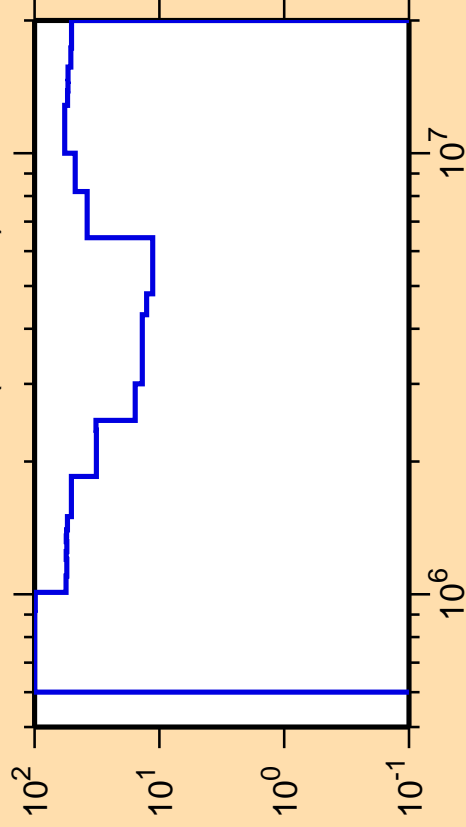
\Delta\sigma/\sigma vs. E for ^{191}\text{Os}(n,n\text{cont.})
