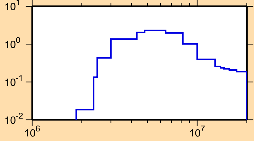
\sigma vs. E for ^{203}\text{Hg}(n,n\text{cont.})
