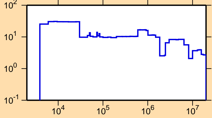
\Delta\sigma/\sigma vs. E for ^{203}\text{Hg}(n,\text{tot.})
