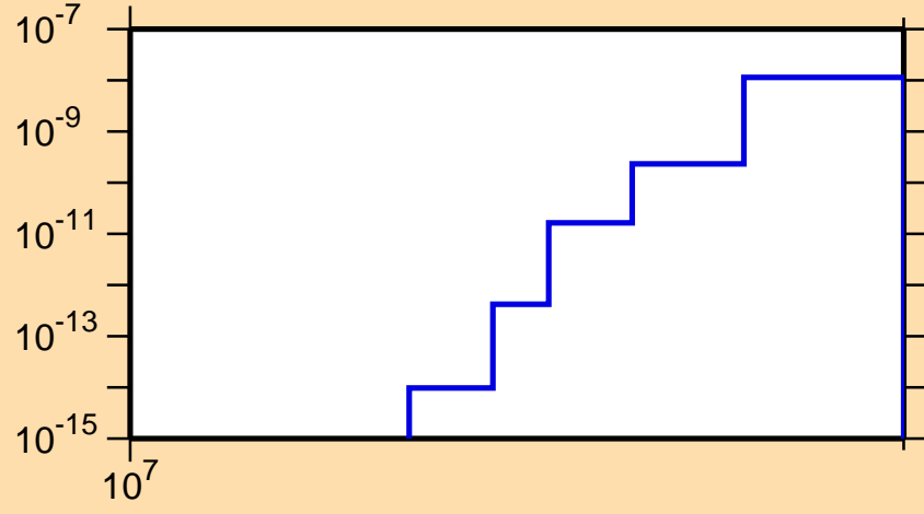
\sigma vs. E for ^{203}\text{Hg}(n,p\alpha)
