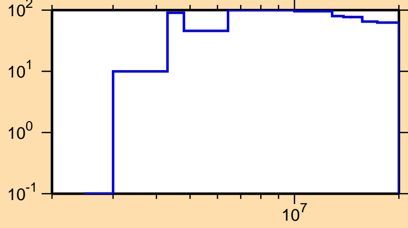
\Delta\sigma/\sigma vs. E for ^{203}\text{Hg}(n,p)
