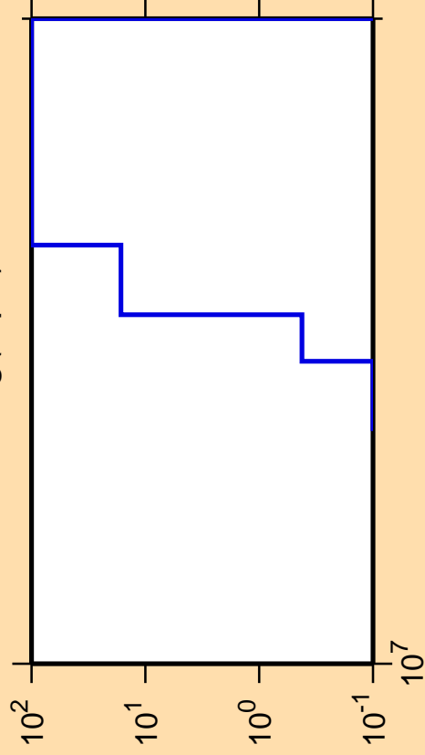
\Delta\sigma/\sigma vs. E for ^{203}\text{Hg}(n,p\alpha)
