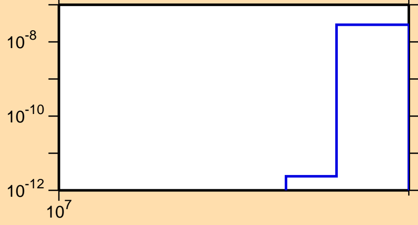
\sigma vs. E for ^{203}\text{Hg}(n,nt)
