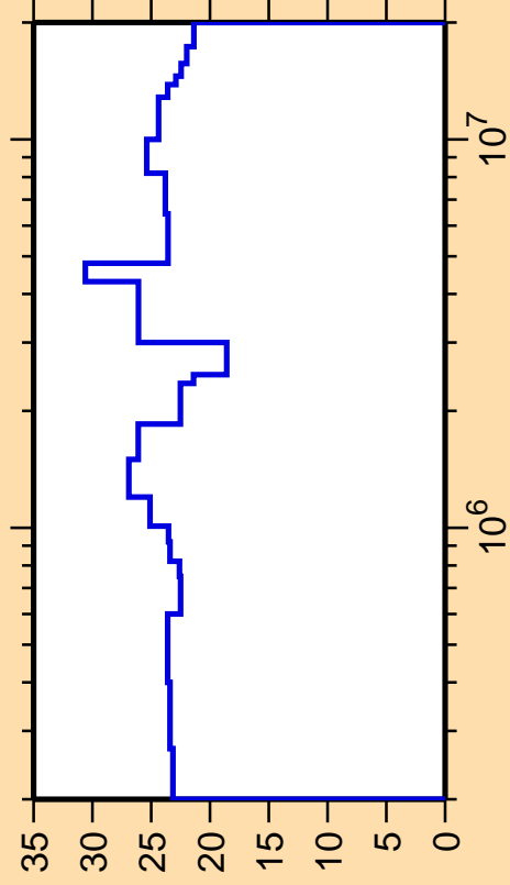
\Delta\sigma/\sigma vs. E for ^{225}\text{Ac}(n,n_{12})
