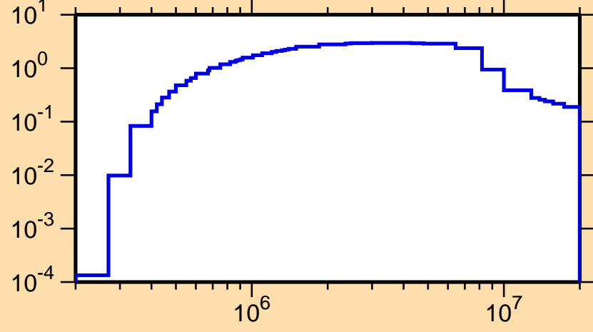
\sigma vs. E for ^{225}\text{Ac}(n,n\text{cont.})
