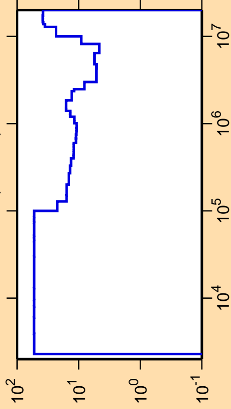
\Delta\sigma/\sigma vs. E for ^{205}\text{Pb}(n,\text{inel.})
