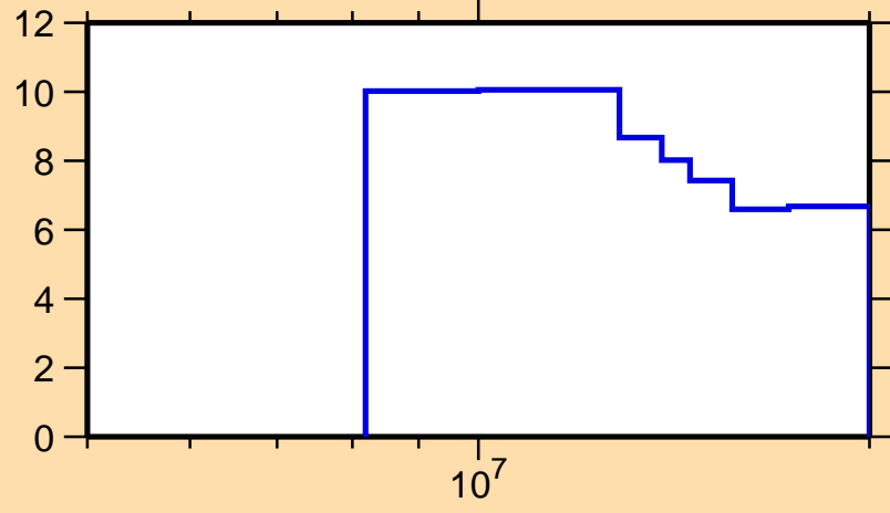
\Delta\sigma/\sigma vs. E for ^{205}\text{Pb}(n,el.)
