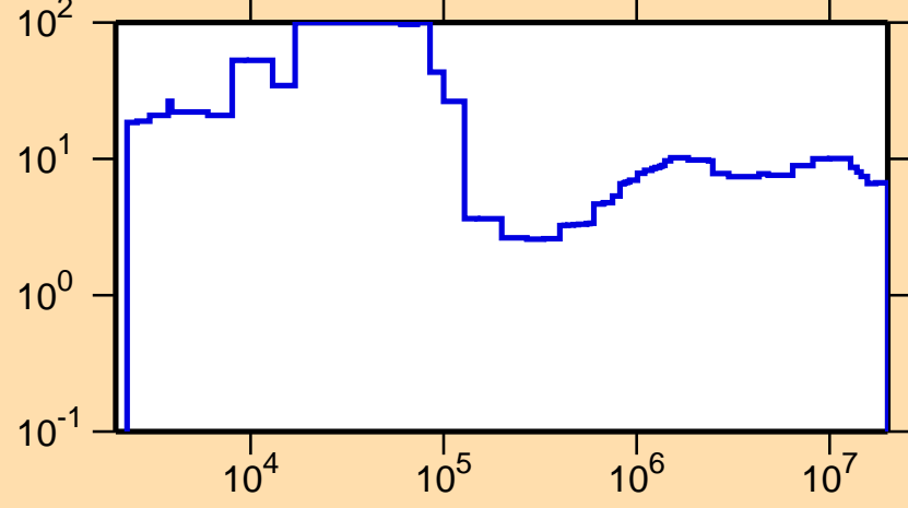
\Delta\sigma/\sigma vs. E for ^{205}\text{Pb}(n,\text{el.})
