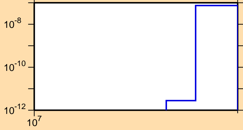
\sigma vs. E for ^{204}\text{Pb}(n,2np)
