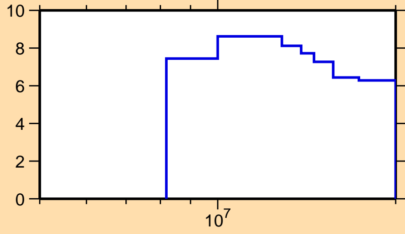
\Delta\sigma/\sigma vs. E for ^{204}\text{Pb}(n,el.)
