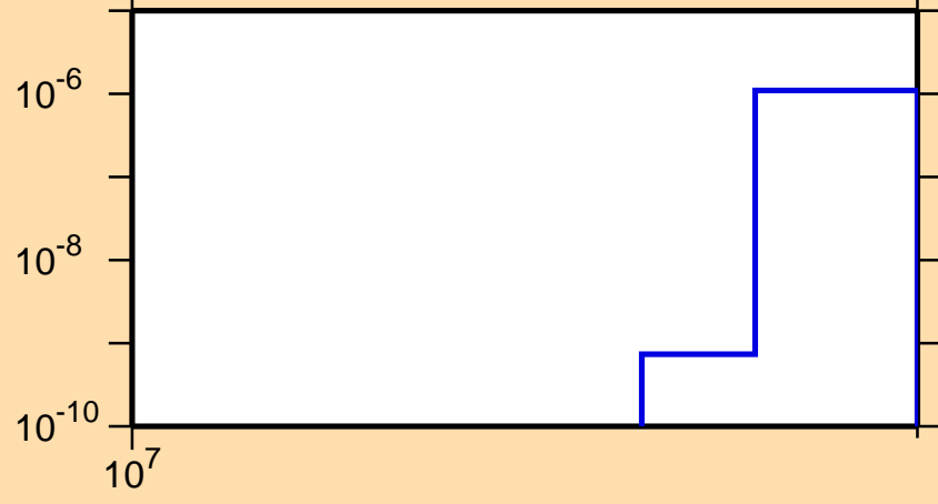
\sigma vs. E for ^{204}\text{Pb}(n,\text{nd})
