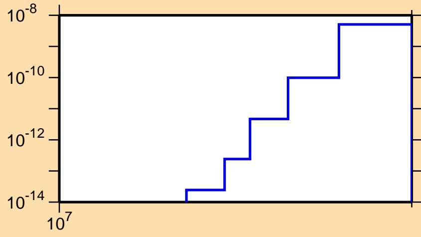
\sigma vs. E for ^{208}\text{Po} (mt 45)
