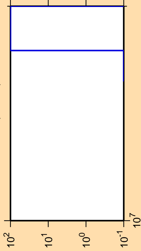
\Delta\sigma/\sigma vs. E for ^{208}\text{Po} (mt 34)
