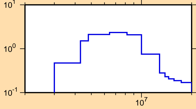
\sigma vs. E for ^{208}\text{Po}(n,n\text{cont.})
