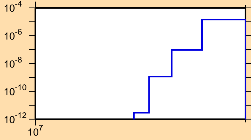
\sigma vs. E for ^{208}\text{Po}(n,\text{nd})
