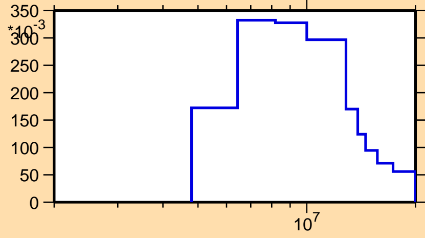
\sigma vs. E for ^{253}\text{Cf}(n,2n)
