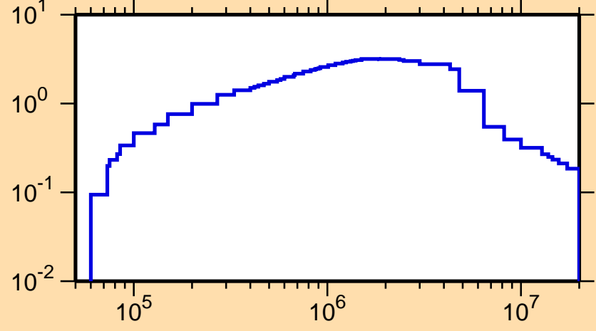
\sigma vs. E for ^{253}\text{Cf}(n,\text{inel.})
