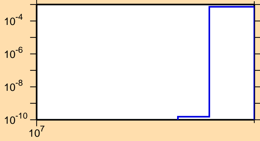
\sigma vs. E for ^{255}\text{Fm}(n,4n)
